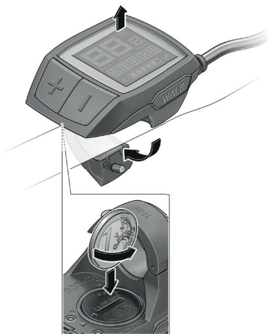
Image 31: Changing the batteries of the Purion display
