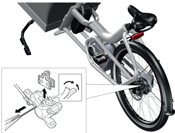
Image 42: Removing the brake pads in order to check them for wear
