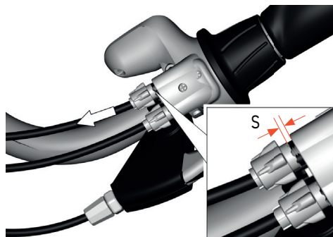
Image 43: Checking cable slack
