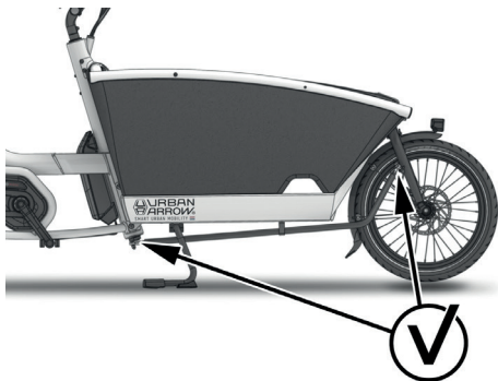
Image 39: Check steering linkage at the ball joints
