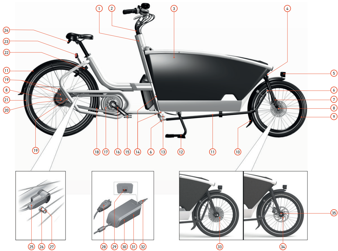
Image 1: General overview (side view)
