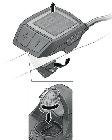
Image 34: Changing the batteries of the Purion display
