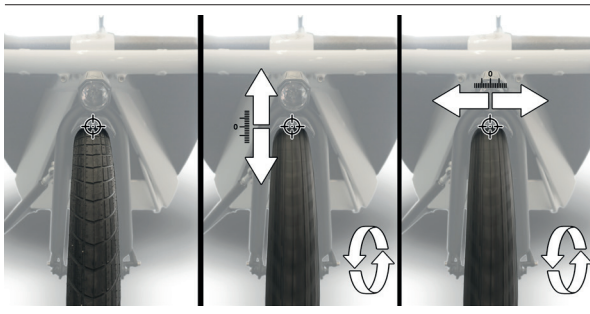
Image 37: Checking the wheel trueness
